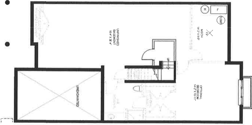
BASEMENT PLAN
