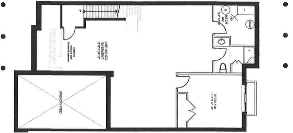
BASEMENT PLAN
