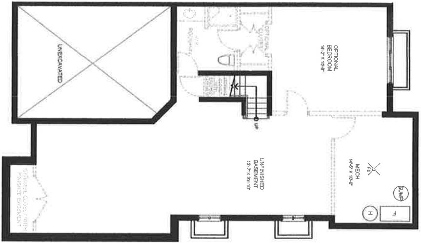
BASEMENT PLAN
